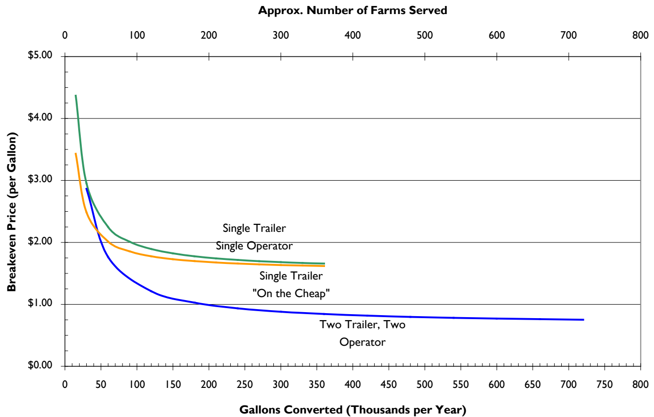
Figure 10: Breakeven Pricing for Biodiesel Conversion.
