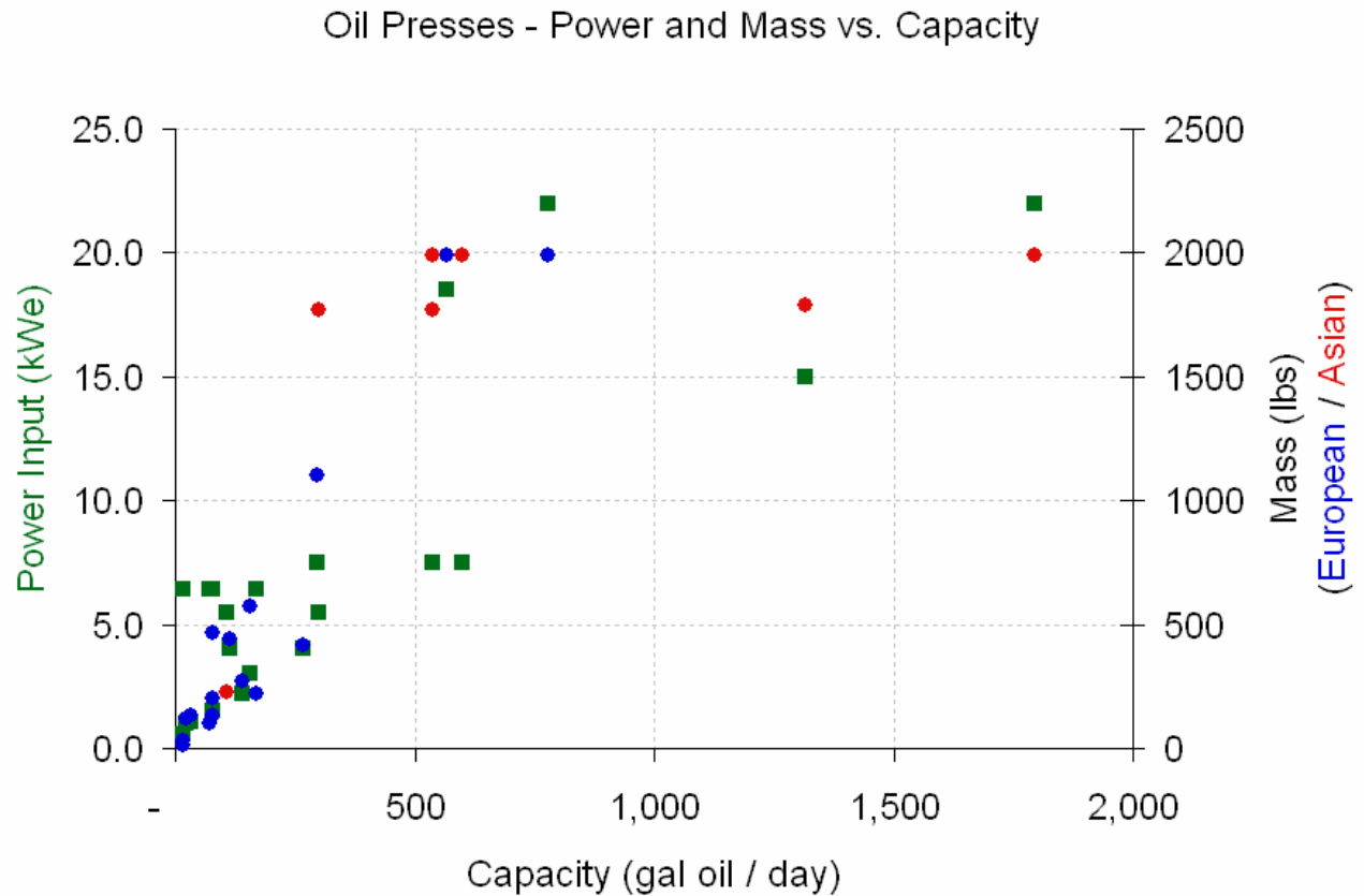
Figure 5: Power Requirements and Mass of Oilseed Presses.
