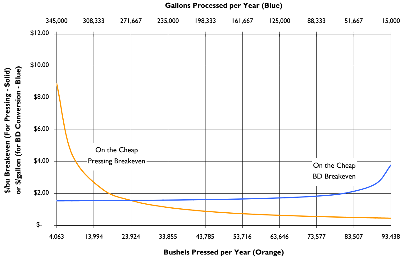
Figure 13: Breakeven Curves for Pressing (Orange) and Biodiesel Conversion (Blue) Assuming the Manual / On the Cheap Model.
