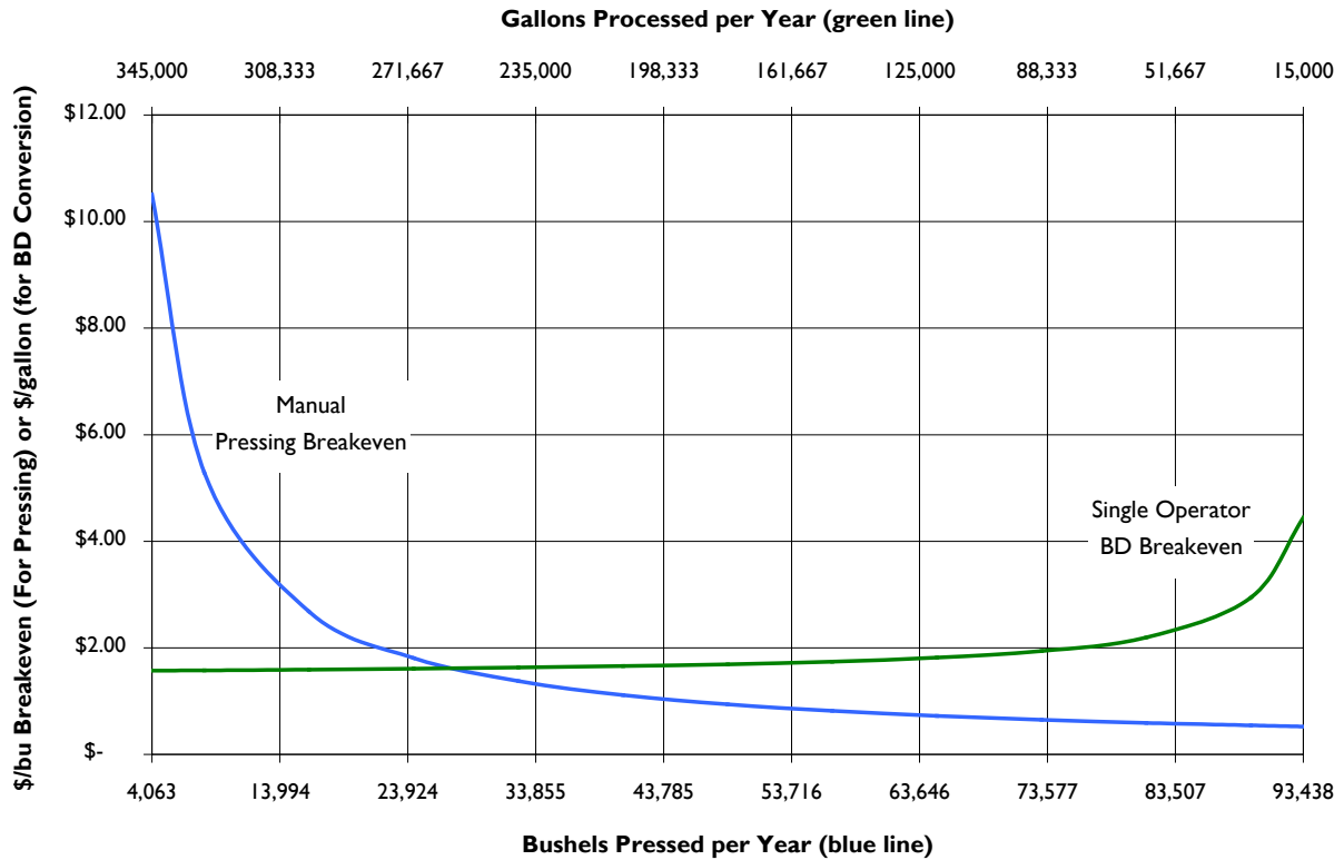
Figure 11: Breakeven Curves for Pressing (Blue) and Biodiesel Conversion (Green) Assuming the Manual / Single Operator Model.
