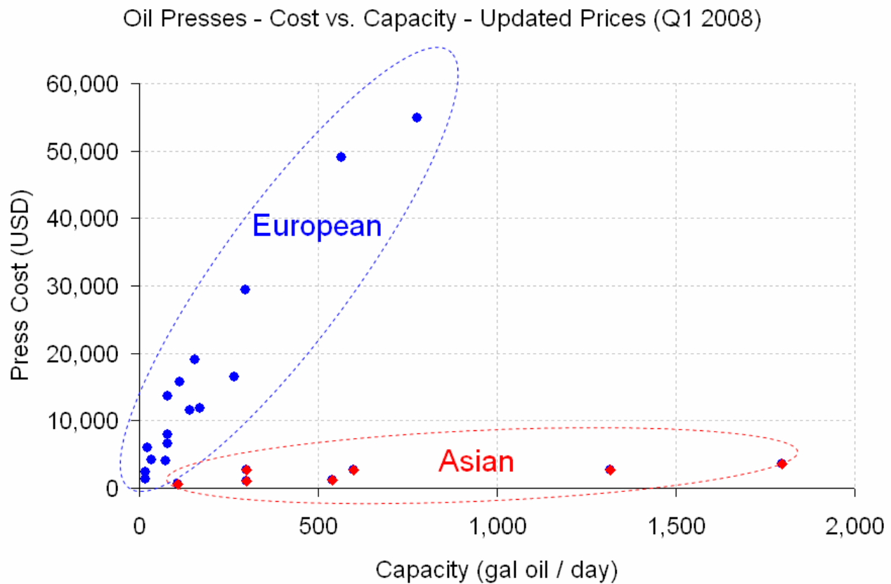
Figure 4: Cost and Capacity of Oilseed Presses.
